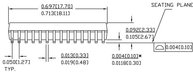
Figure 14. 28-Pin (330 mil) SOIC (51-85058)
