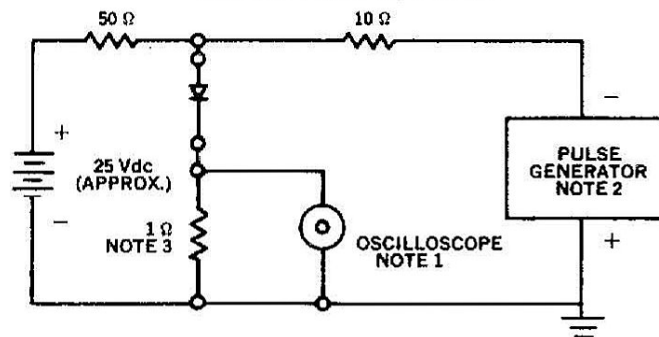
Reverse-Recovery Circuit
