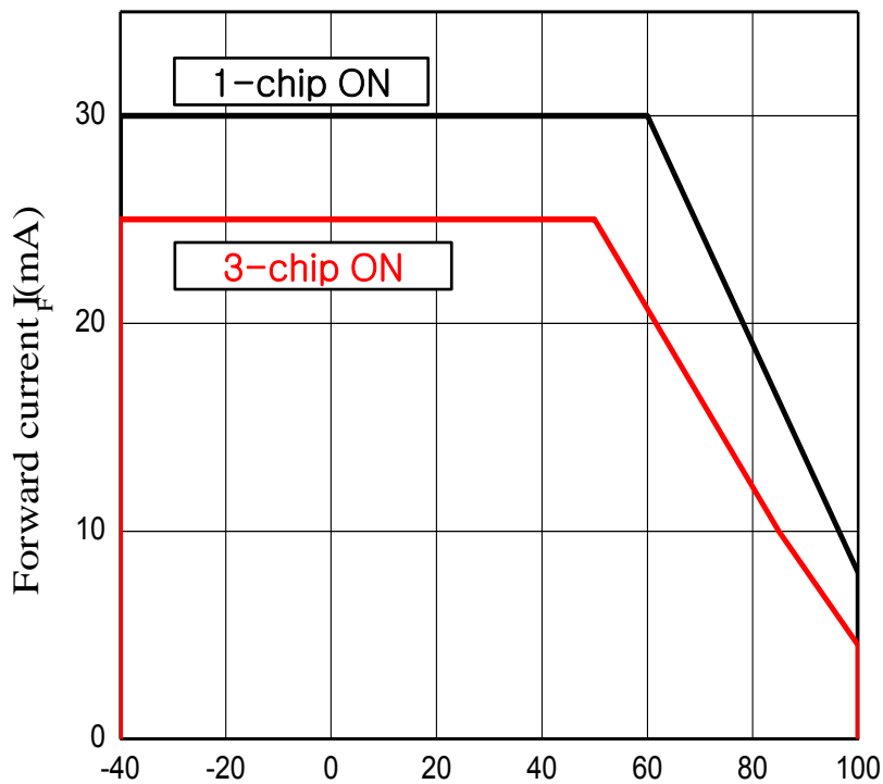
Fig 4. Forward Current vs. Derating Curve, T_a=25^\circ\text{C}
