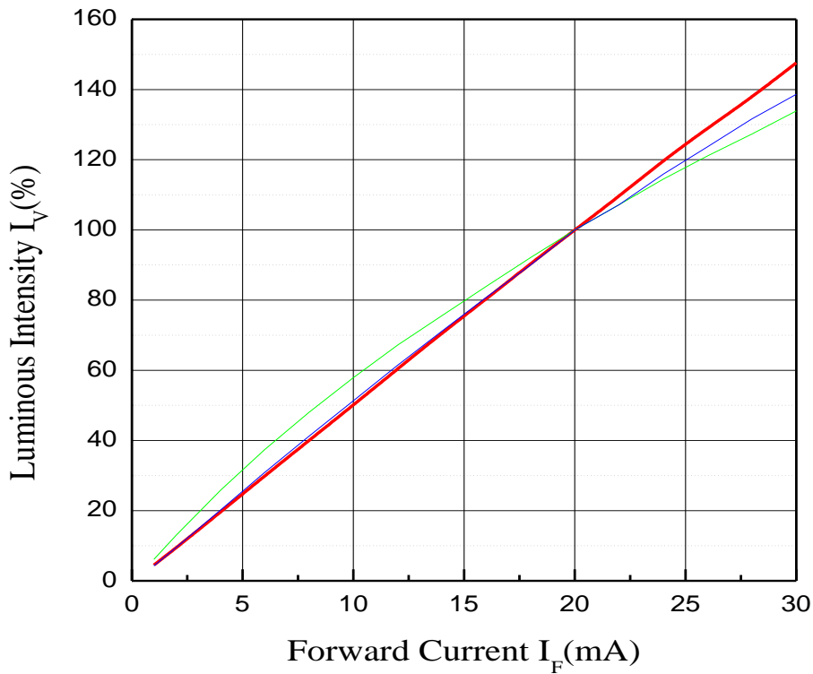
Fig 2. Relative Intensity vs. Forward Current, T_a=25^\circ\text{C}
