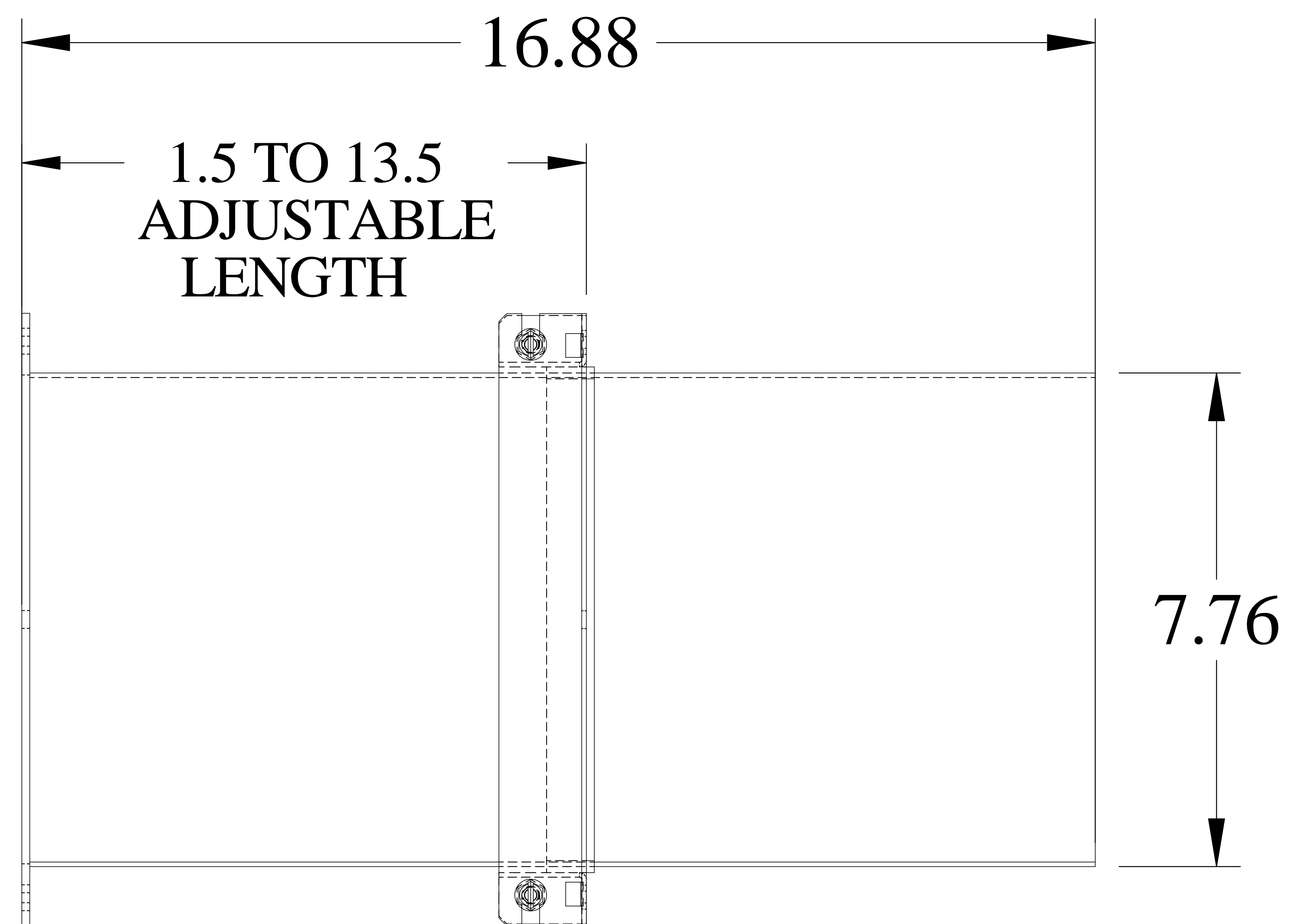
SIDE VIEW
