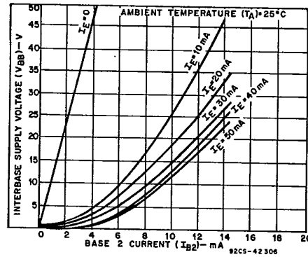
Fig. 5—Typical static interbase characteristics.
