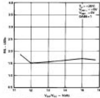
Figure 13. Typical Linearity vs. V_{DD}/V_{DDT}
