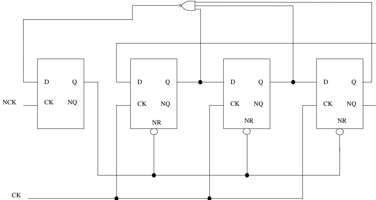
Figure 2. Correct Construction of a Divide-by-3 Counter
