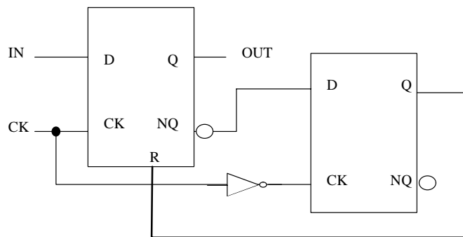
Figure 3. If Must Make Pulses, Do It This Way
