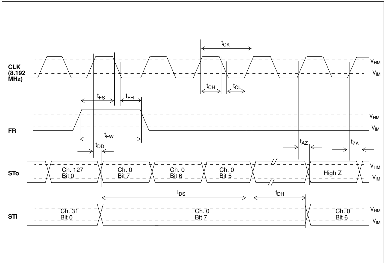
Figure 24 - Rate Conversion Mode (DMO bit=1) - 2 Mb/s to 8 Mb/s
