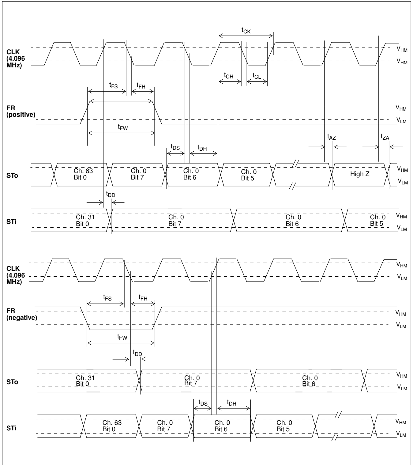
Figure 21 - Rate Conversion Mode (DMO bit=1) - 4 Mb/s to 2 Mb/s
