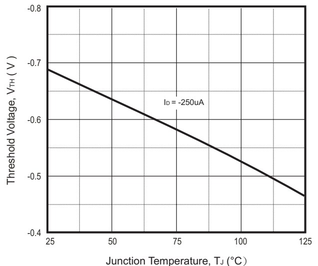
Fig.6 - Threshold Voltage
