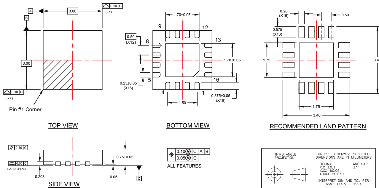
Figure 26. Package Drawing 16-lead 3 × 3 mm QFN
