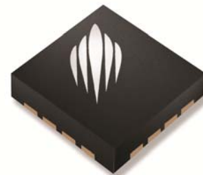
Figure 2. Package Type 16-lead 3 × 3 mm QFN
