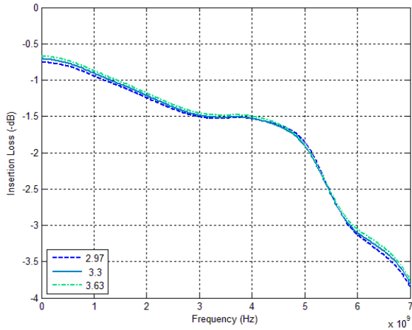
Figure 4. Differential Insertion Loss over V_{DD}
