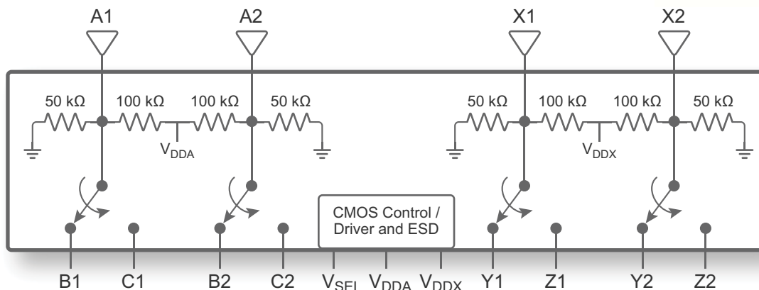
Figure 1. Functional Diagram
