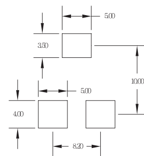
Suggested Land Pattern
