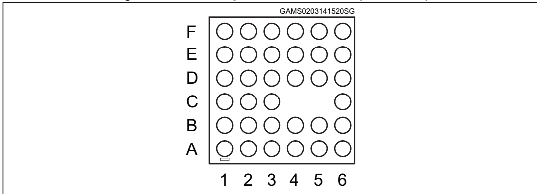
Figure 4. BlueNRG pinout bottom view (WLCSP34)
