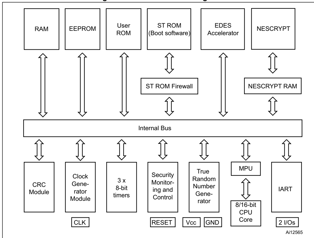
Figure 1. ST23YL48 block diagram
