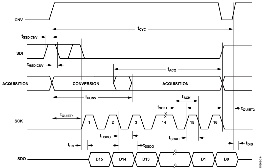
Figure 57. CS Mode, 4-Wire Turbo Mode Timing Diagram
