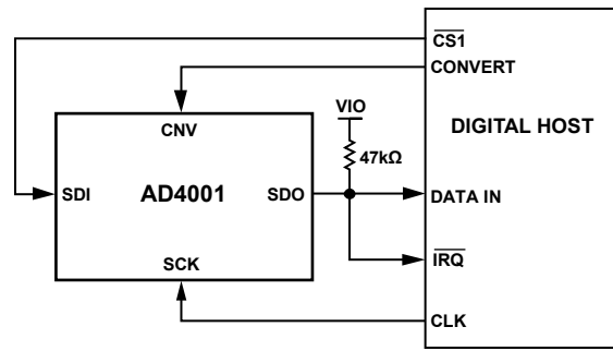
Figure 56. CS Mode, 4-Wire Turbo Mode Connection Diagram
