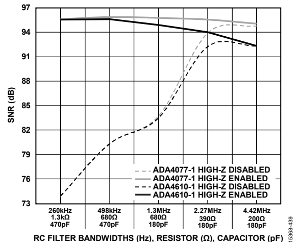
Figure 42. SNR vs. RC Filter Bandwidth for Various Precision ADC Drivers, V_{REF} = 5\text{ V} , f_{IN} = 1\text{ kHz} (Turbo Mode On, High-Z Enabled/Disabled), V_{IO} = 3.3\text{ V}
