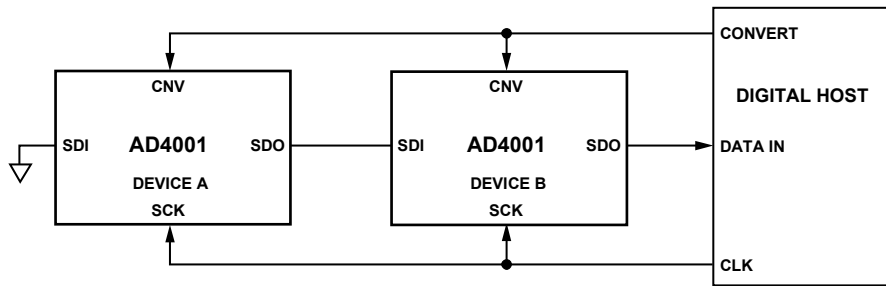
Figure 62. Daisy-Chain Mode Connection Diagram
