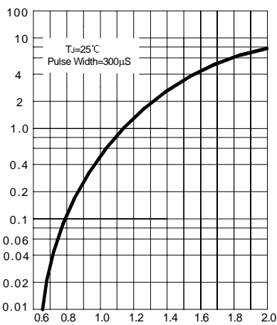
FIG.4–TYPICAL FORWARD CHARACTERISTIC
