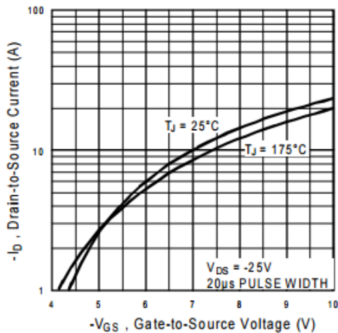
Fig. 3 Typical Output Characteristics, T_C = 150^{\circ}C
