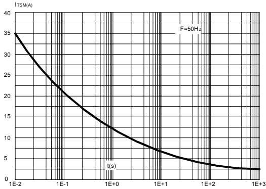
FIG.1 – NON REPETITIVE SURGE PEAK ON-STATE CURRENT VERSUS OVERLOAD DURATION ( T_J IN |t| = 25°C).
