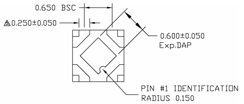
BOTTOM VIEW
