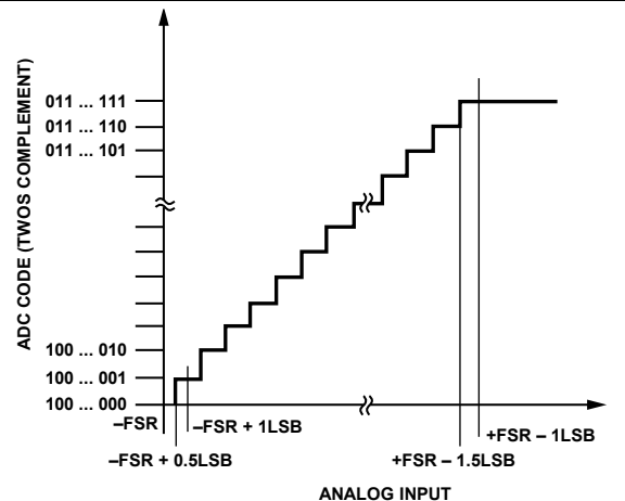
Figure 91. Transfer Function
