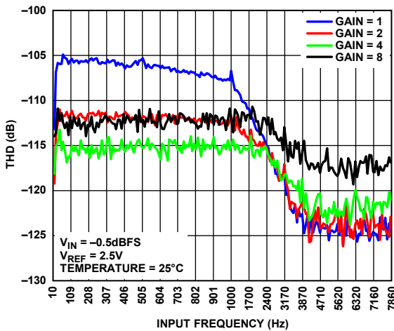
Figure 28. THD vs. Input Frequency at 16 kSPS, High Resolution Mode
