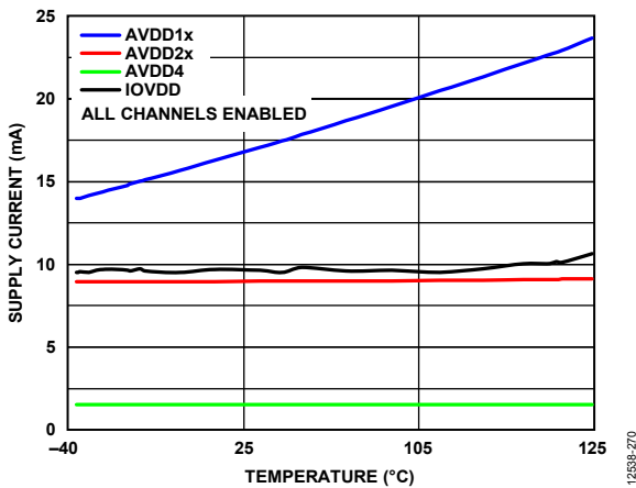
Figure 70. Supply Current vs. Temperature, High Resolution Mode
