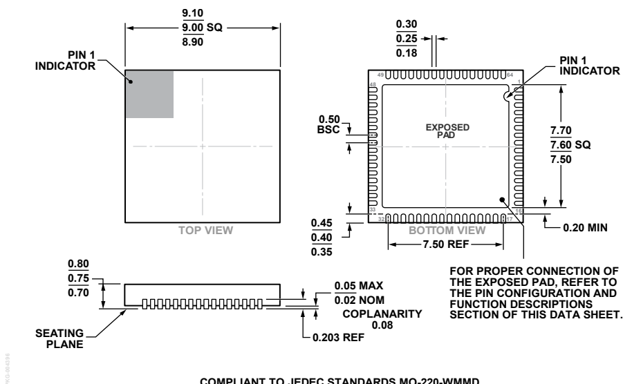
Figure 121. 64-Lead Lead Frame Chip Scale Package [LFCSP] 9 mm × 9 mm Body and 0.75 mm Package Height (CP-64-15)
