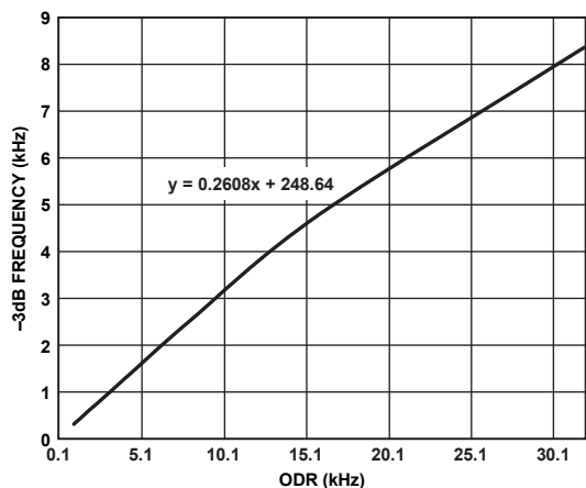
Figure 111. -3 dB Correction Factor
