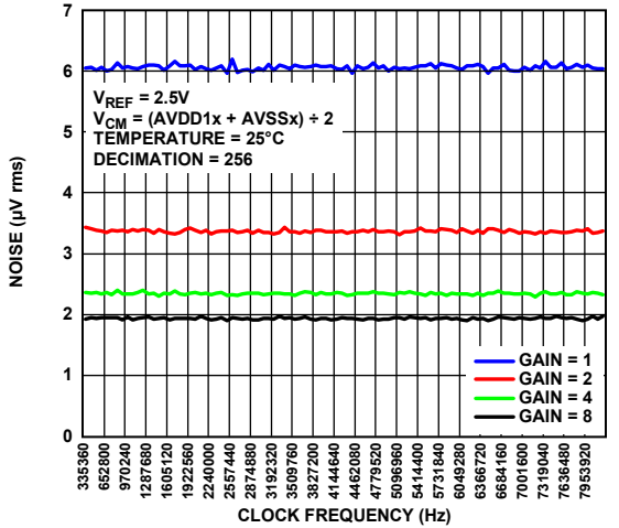
Figure 21. Noise vs. Clock Frequency, High Resolution Mode
