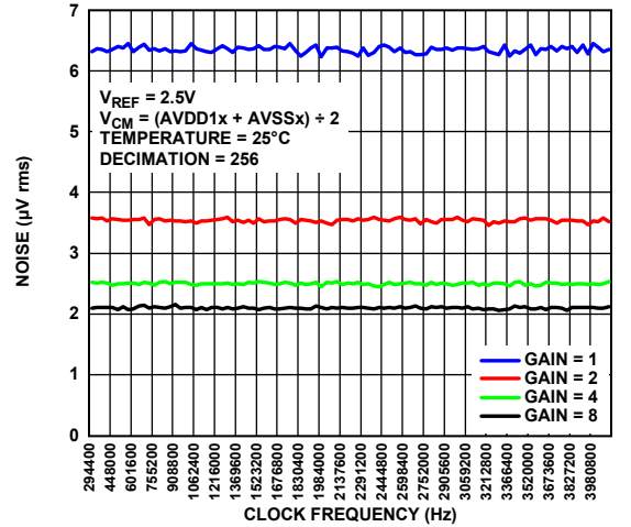
Figure 24. Noise vs. Clock Frequency, Low Power Mode
