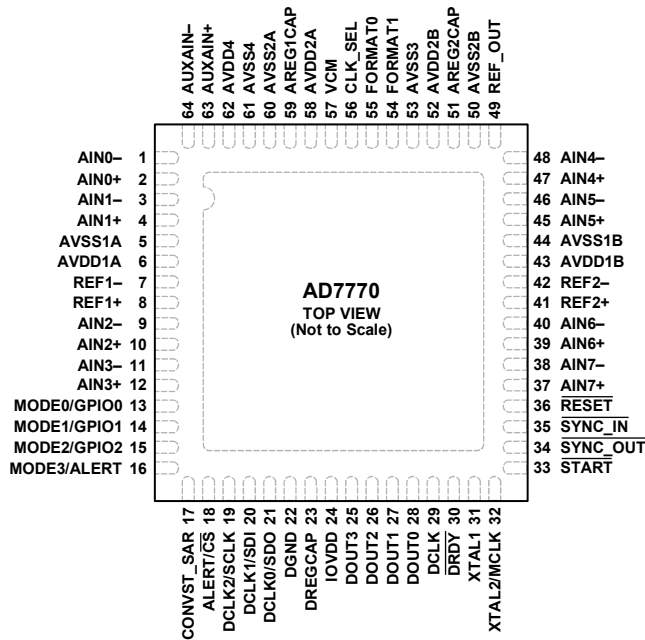
Figure 7. Pin Configuration
