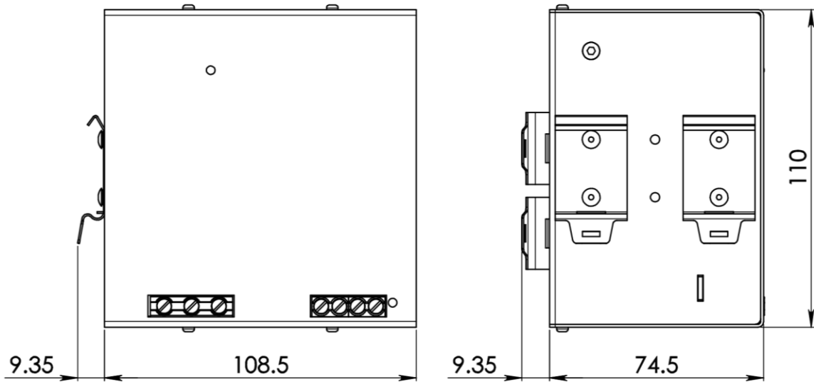
Figure 1. Mechanical Drawing
