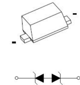
SOD-523
