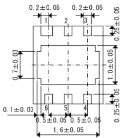
USP-6B Reference Metal Mask Design, Units: mm
