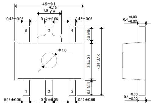
SOT-89-5, Units: mm
