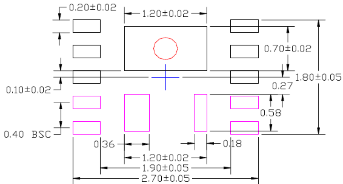
10-Pin 2.5mm x 2mm MLF®
