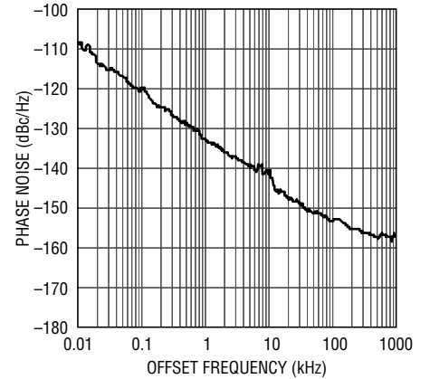
Additive Phase Noise, f_{OUT} = 65MHz , f_{DAC} = 2.7Gps
