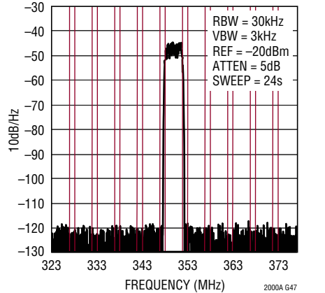
LTC2000A-16 Single Carrier WCDMA ACLR at 350MHz, f_{DAC} = 2.7Gps
