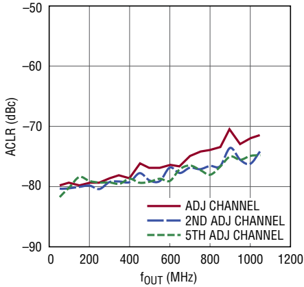
LTC2000A-16 Single Carrier WCDMA ACLR vs f_{OUT} , f_{DAC} = 2.7Gps
