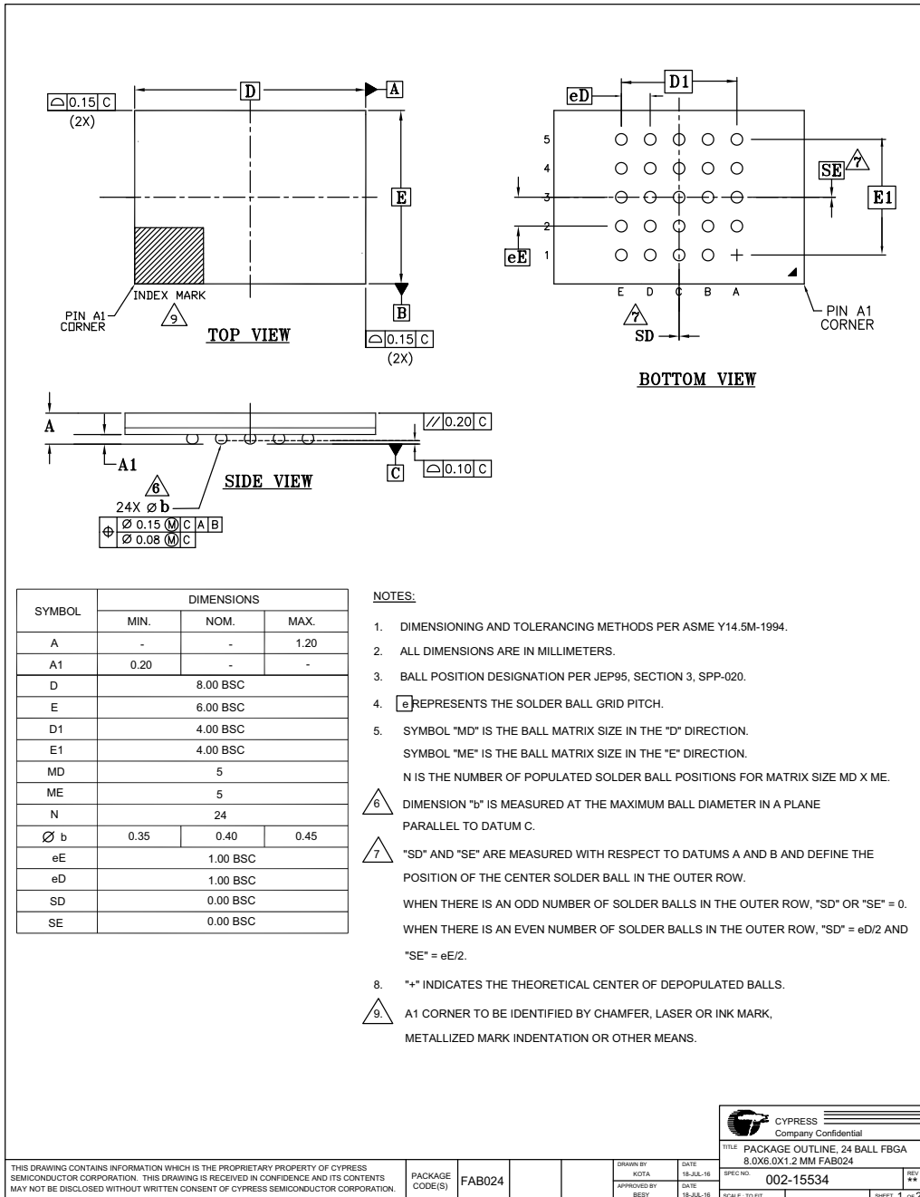
Figure 41. Ball Grid Array 24-Ball 6x8 mm (FAB024)
