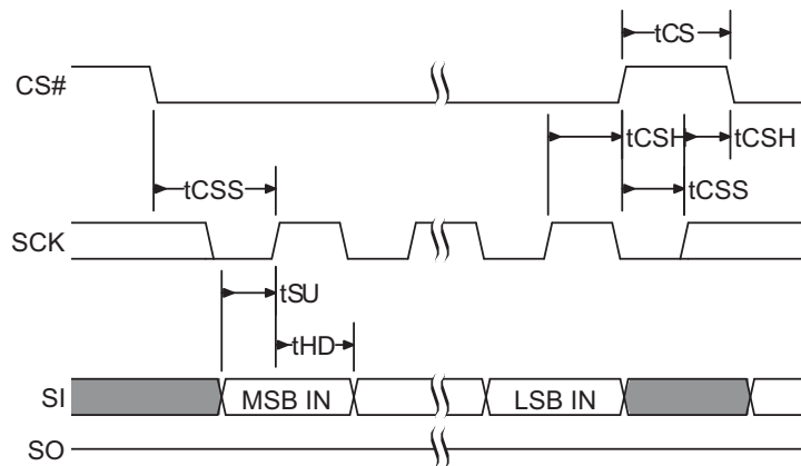
Figure 29. SPI Single Bit Input Timing
