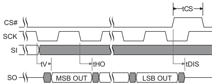
Figure 30. SPI Single Bit Output Timing
