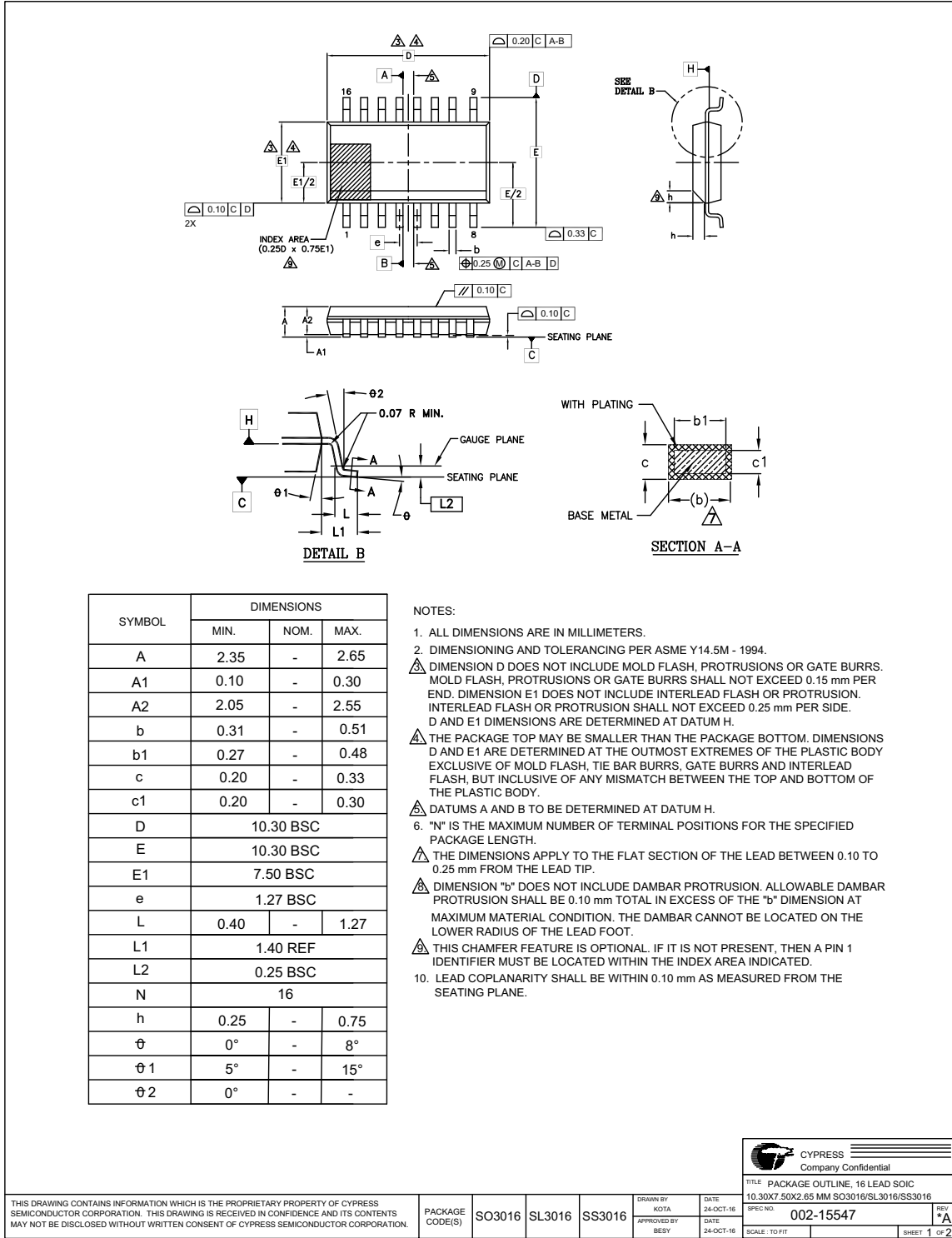
Figure 37. SOIC 16-Lead, 300-mil Body Width (SO3016)
