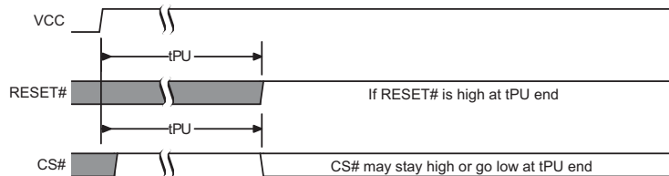
Figure 25. POR followed by Hardware Reset
