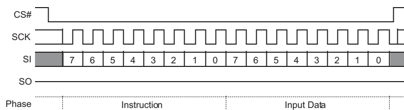
Figure 72. Set Burst Length Command Sequence
