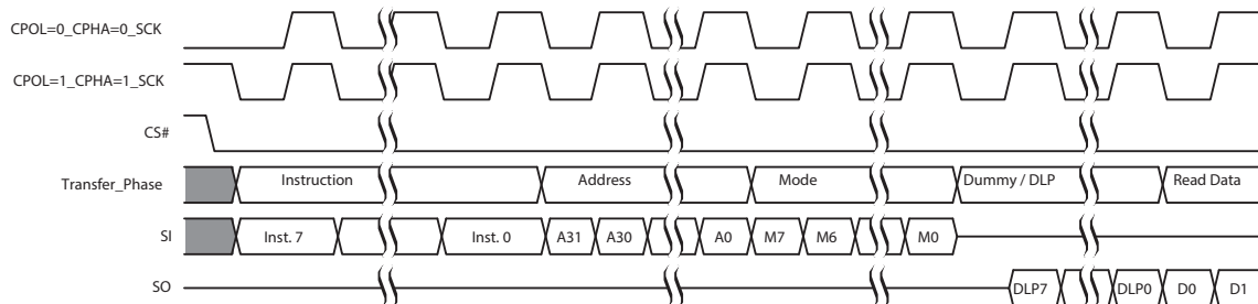
Figure 5. SPI DDR Modes Supported
