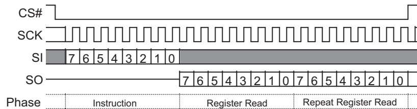
Figure 68. DLP Read (DLPRD) Command Sequence
