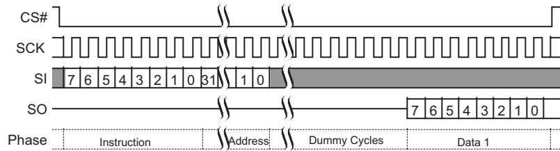
Figure 11. Dual I/O Command
