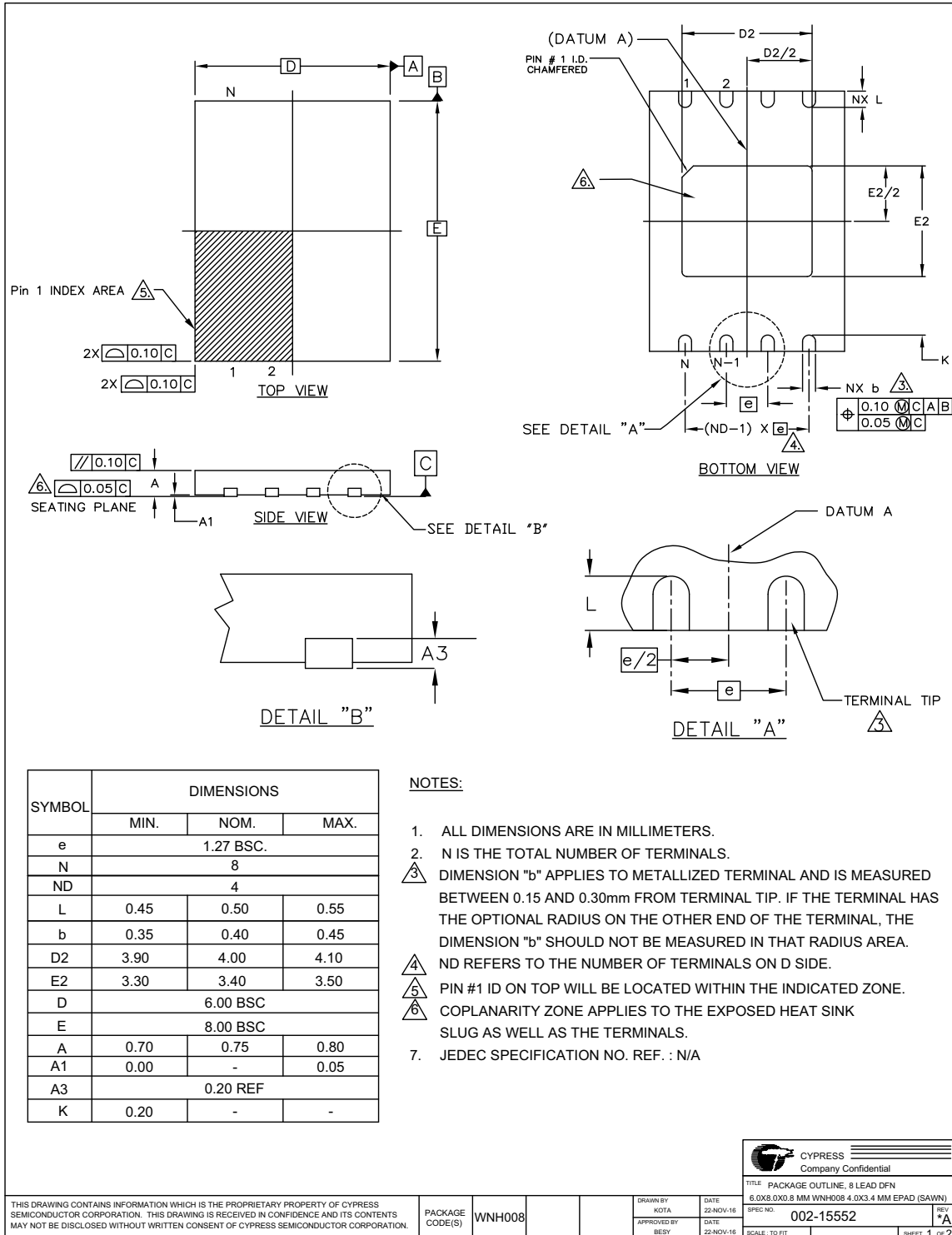
Figure 39. WSON 8-Contact 6x8 mm Leadless (WNH008)
