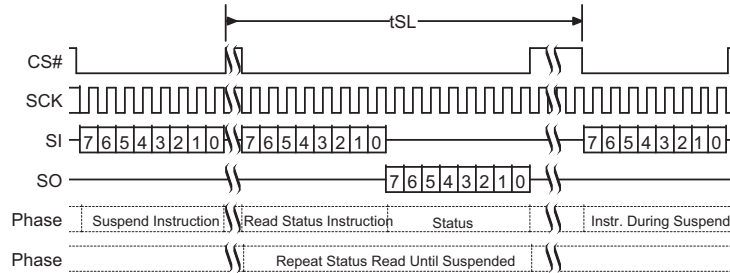
Figure 93. Program or Erase Suspend Command Sequence
