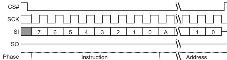
Figure 85. Parameter Sector Erase (P4E 20h or 4P4E 21h) Command Sequence
