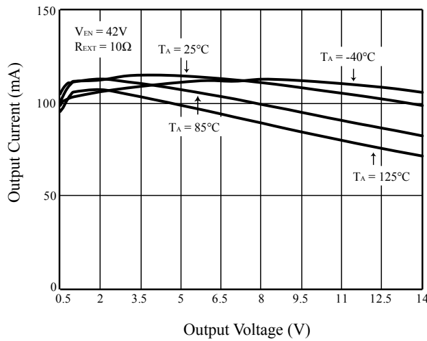
Figure 4 I OUT vs. V OUT
