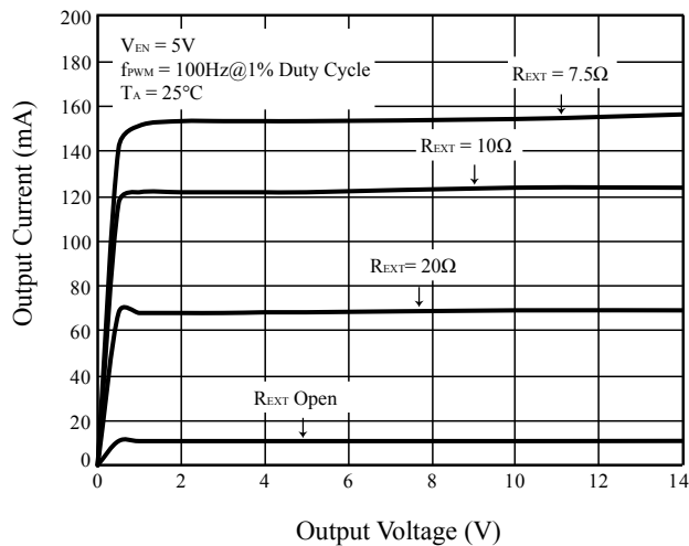
Figure 6 I OUT vs. V OUT
