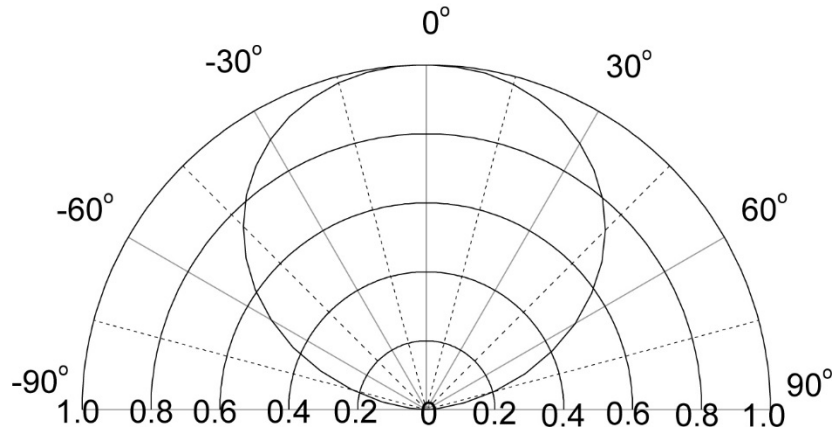
Figure3. Relative Luminosity VS. Radiation Angle
