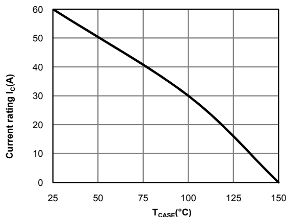
Fig 11: Current De-rating
