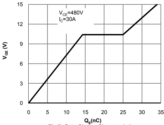
Fig 7: Gate-Charge Characteristics
