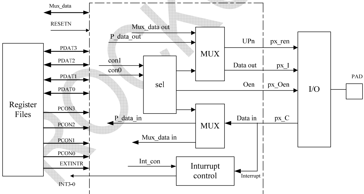
Figure 2. Block Diagram
