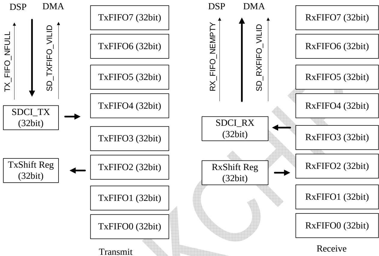
Fig 5. FIFO Block
