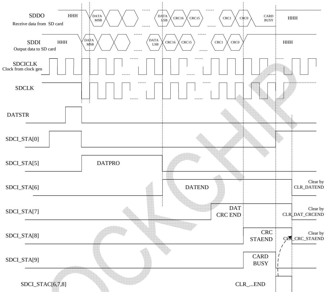
Fig4. Data transmit/recv Timing
