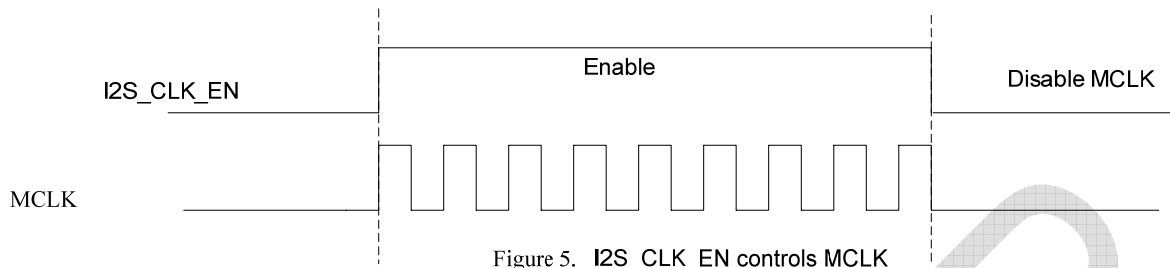
Figure 5. I2S_CLK_EN controls MCLK
