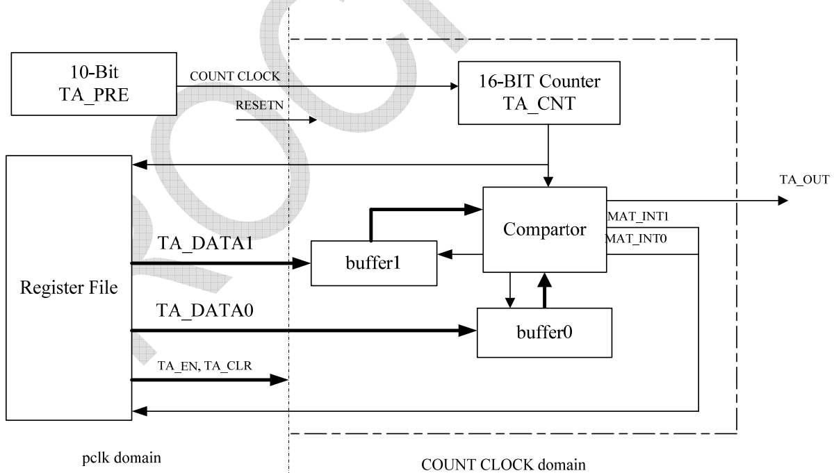
Figure 2. Block Diagram
